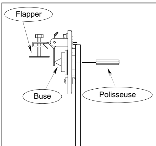
Fig. 6.2.2 "NETTOYAGE BUSE"
