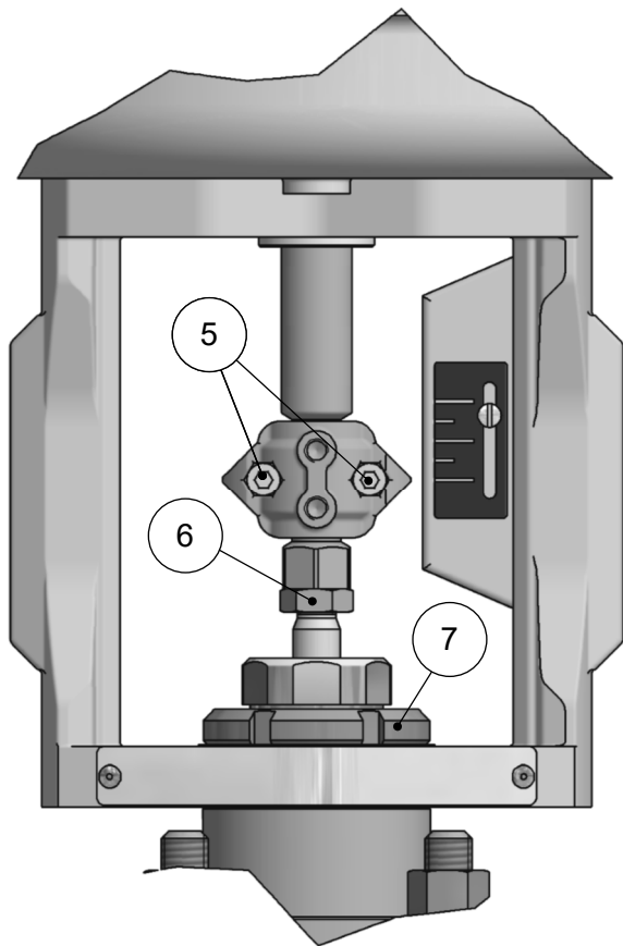
Pic. 17 Valves 1/2" ÷ 2"
